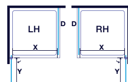
Pivot Door with Side Panel
