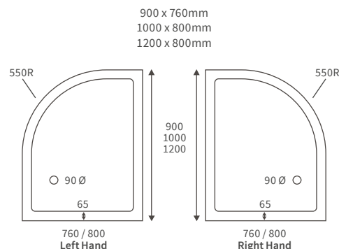
LOW PROFILE OFFSET QUADRANT TRAYS
