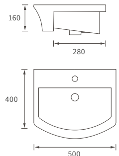
SEMI RECESSED BASIN
