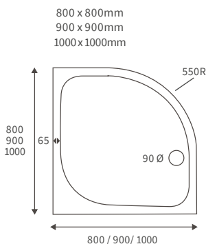
LOW PROFILE QUADRANT TRAYS
